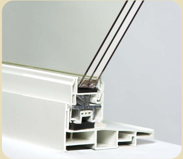
Tribute crosscut featuring triple glazing
